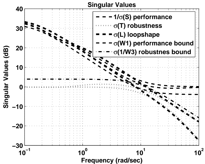
MIXSYN Design Results for NASA HiMAT
